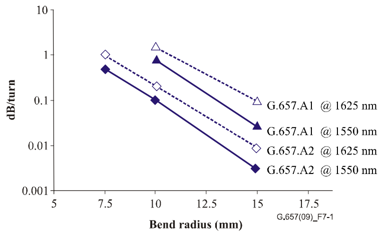
Figure 7-1 – Macrobending loss data from Tables 7-1, category A
