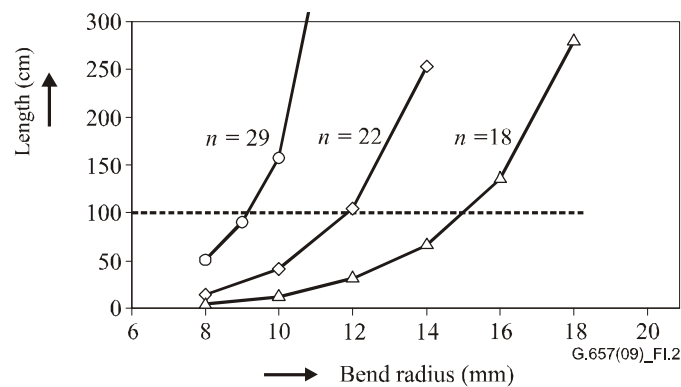
Figure I.2 – Maximum storage length for a bent fibre and different values of the fatigue parameter, n
