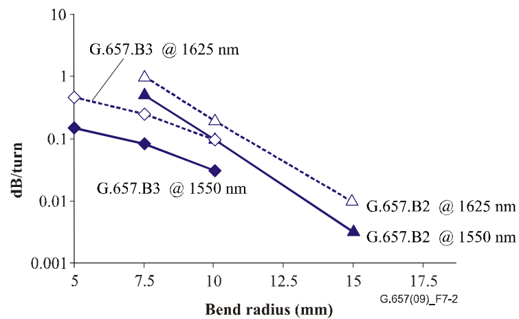
Figure 7-2 – Macrobending loss data from Tables 7-2, category B
